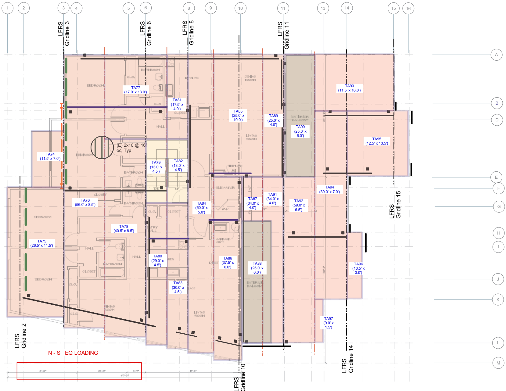
LEVEL 4-R PLAN - N-S TRIBUTARY AREAS
