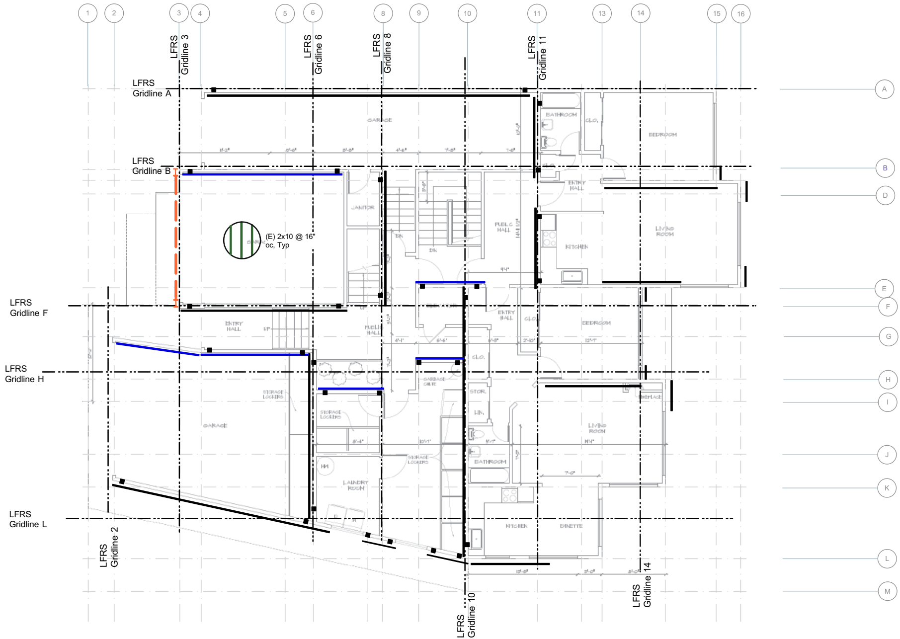
(E) THIRD FLOOR PLAN
