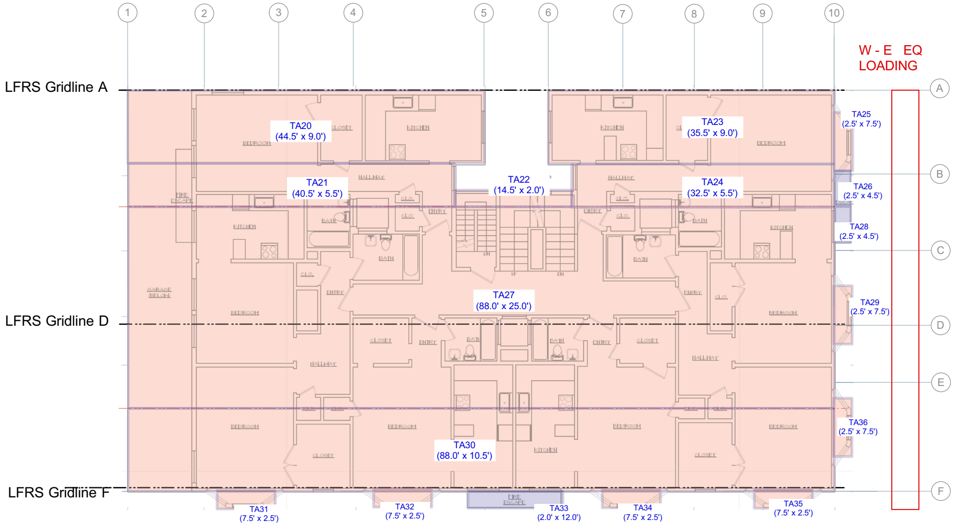
FIRST FLOOR W-E TRIBUTARY AREAS NTS
